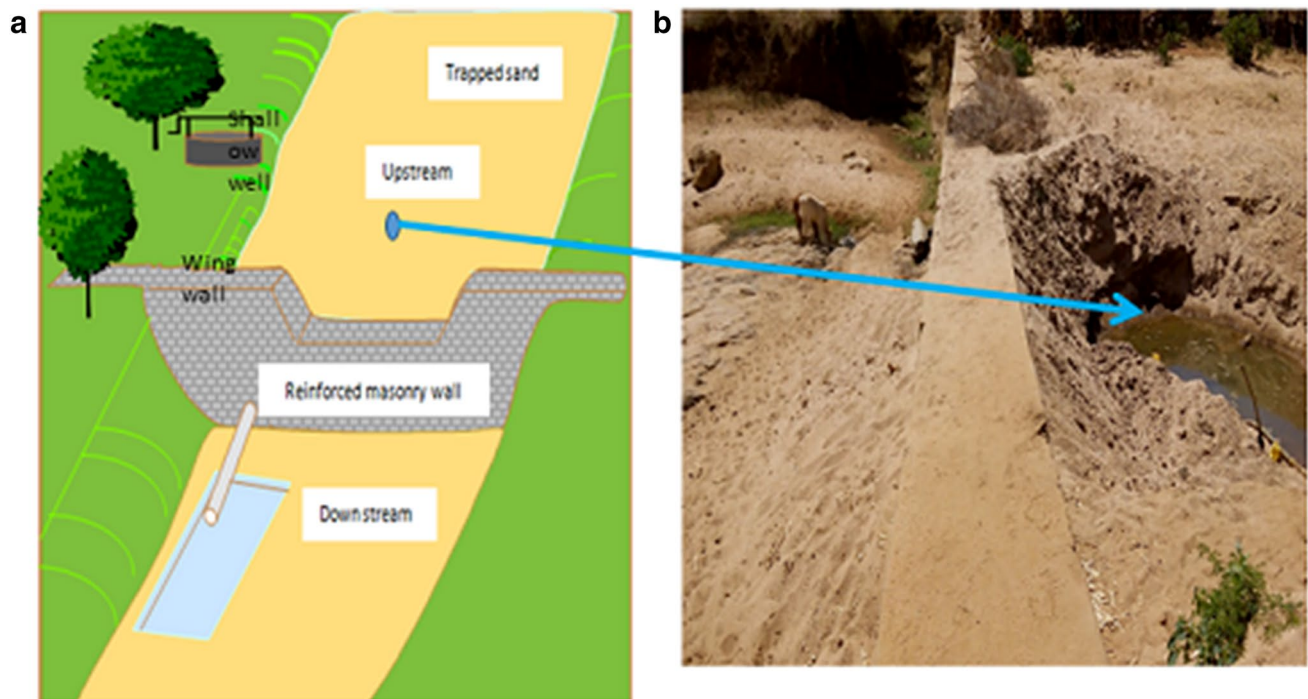
Fig. 1 a and b Sand-storage dam (Left image from (Ngugi 2002), right image was taken by Ngugi in October 2016)
