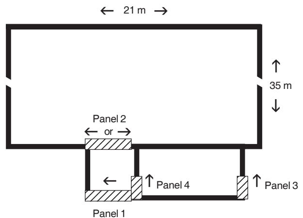
Fig. 6. Diagram of nethouse opening; arrows indicate directions that doors (indicated by slanted boxes) slide
