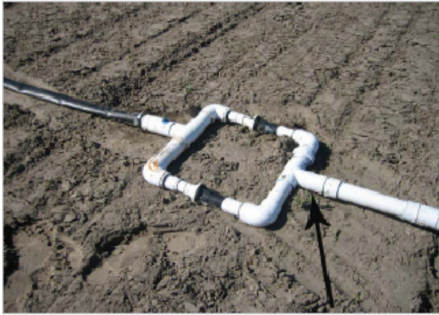
Figure 6. Pressure regulators installed side-by-side allow a greater flow rate.
