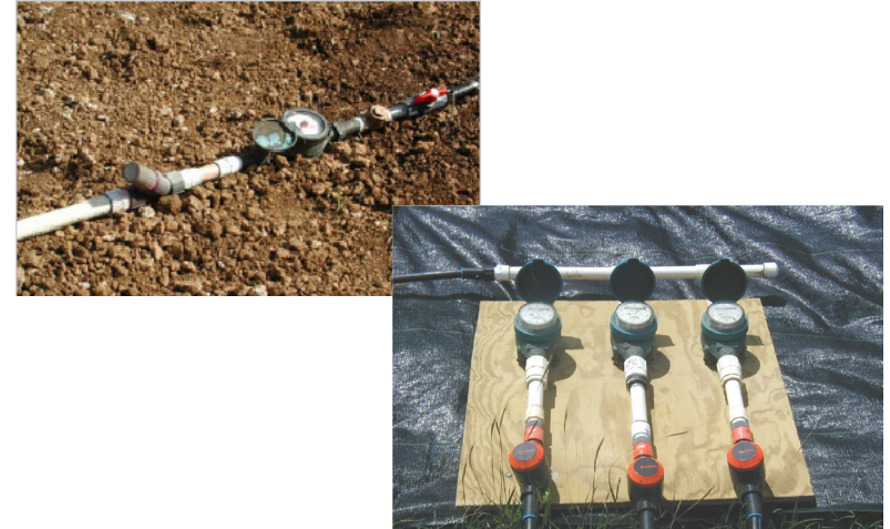
Figure 9. (l) Water meter installed near the field; (r) water meter and timer to control flow of irrigation water.
