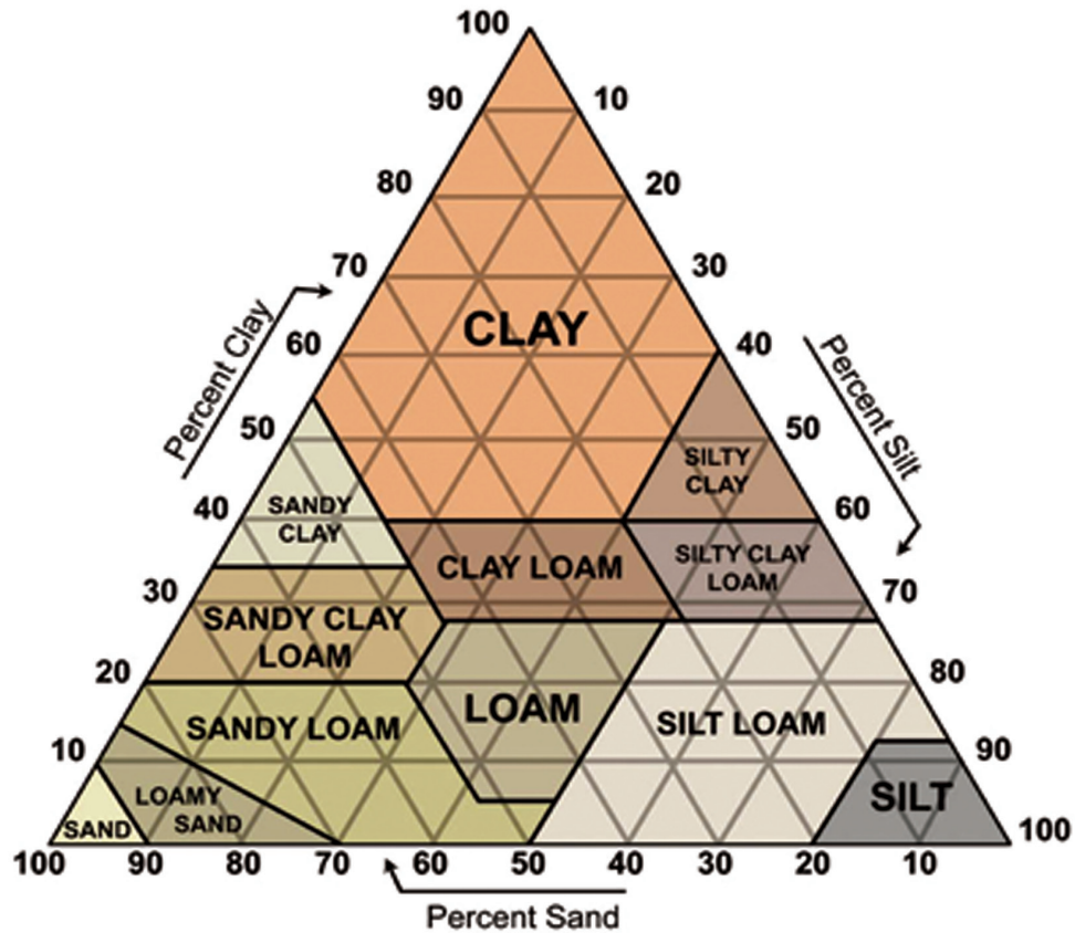
Figure 28. Soil texture triangle. (NSW DPI, 2008a)
