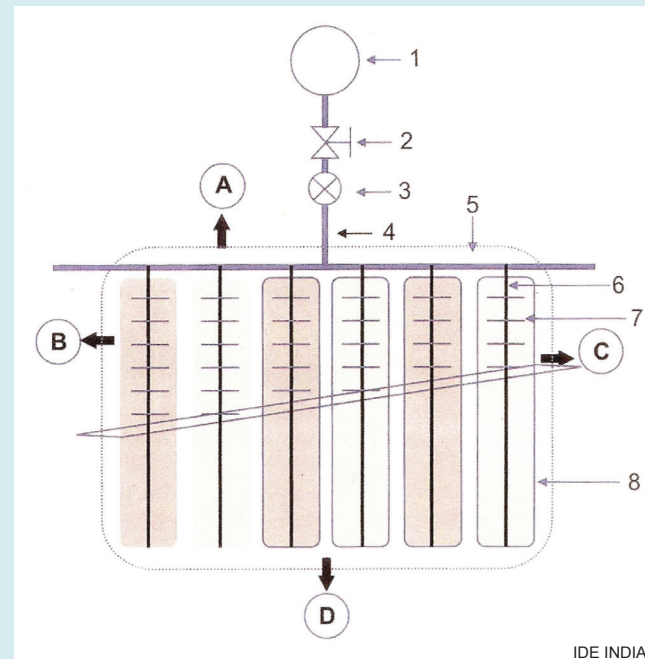
Figure 1. Layout of a typical drip irrigation system
